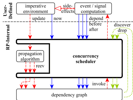
Fig. 7. Layered view of Fig. 3 with added scheduler.
