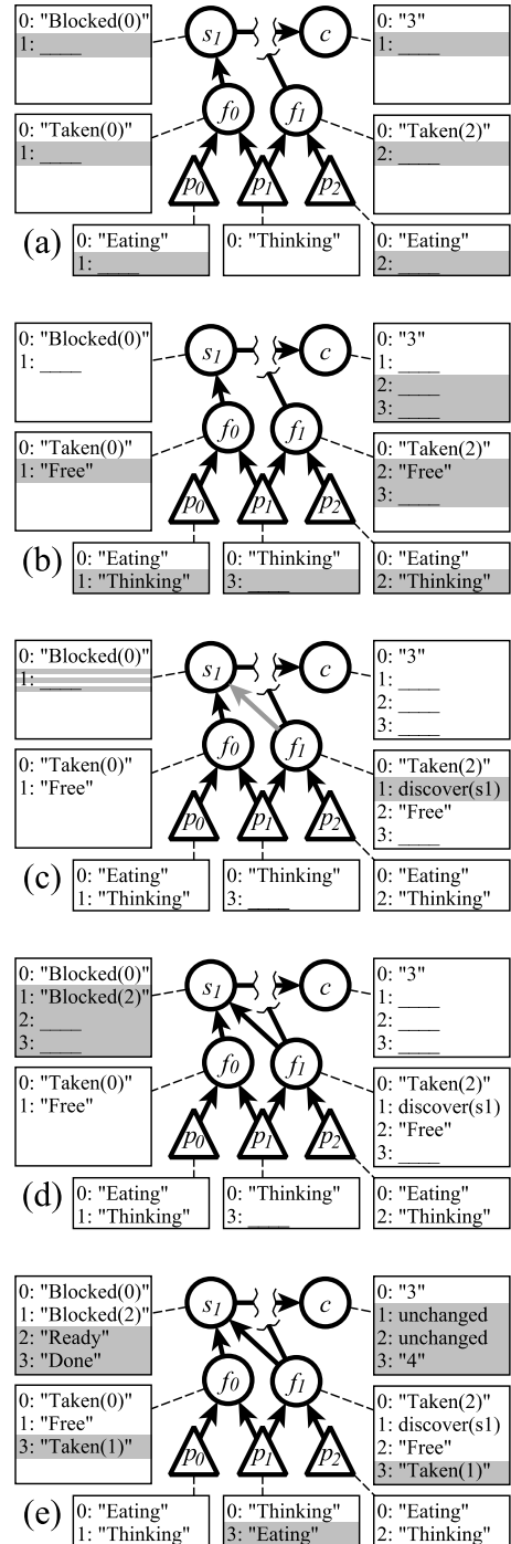
Fig. 8. MV-RP philosopher execution example.
