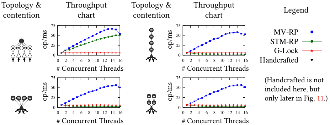
Fig. 9. Scalability across base topologies of updates with approx. 160 \mu\text{s} user computation time.
