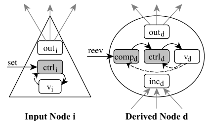
Fig. 4. Composition of reactive nodes.
